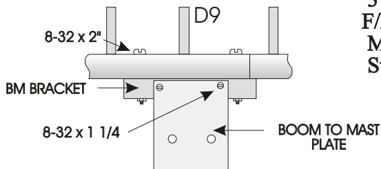
BM BRACKET DETAIL
